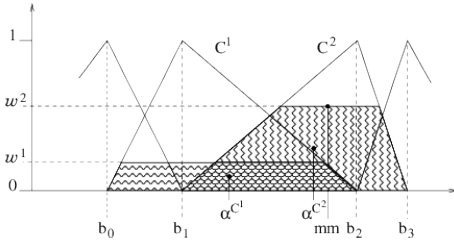
Figure 5: Defuzzification
